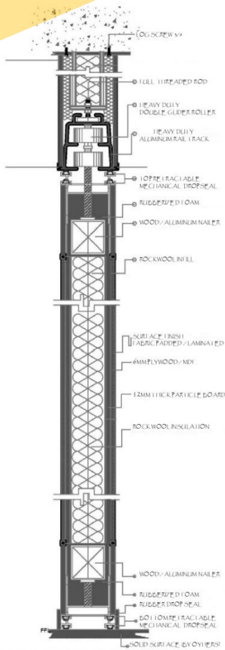
VERTICAL SECTION
