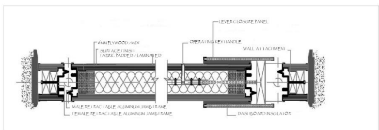
HORIZONTAL SECTION DETAILS
