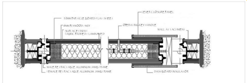
HORIZONTAL SECTION DETAILS
